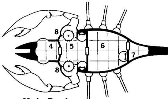
Main Deck
